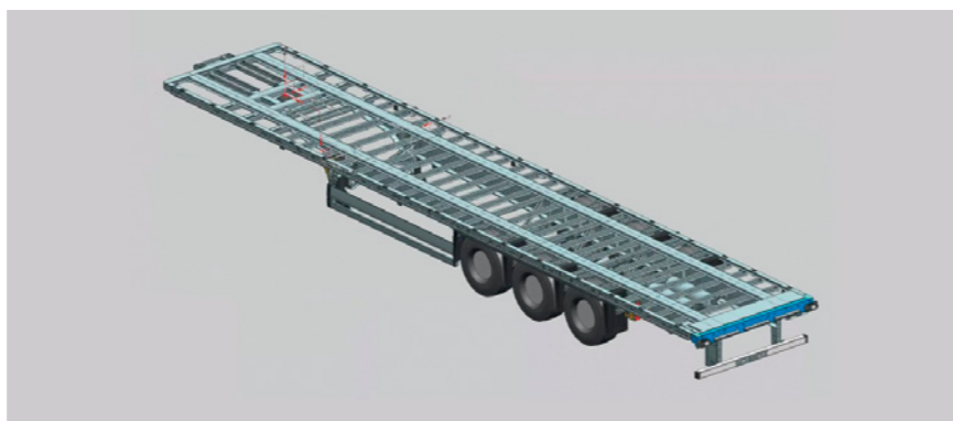
The X-TOUGH chassis impresses with its high bending and torsional strength.
